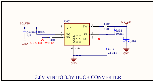
3.8V VIN TO 3.3V BUCK CONVERTER
