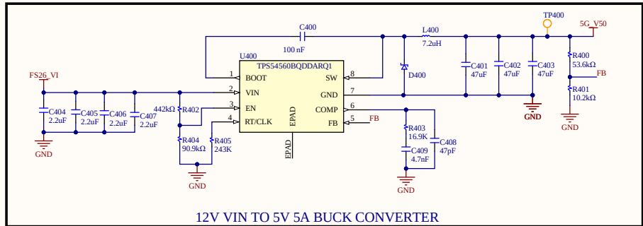
12V VIN TO 5V 5A BUCK CONVERTER
