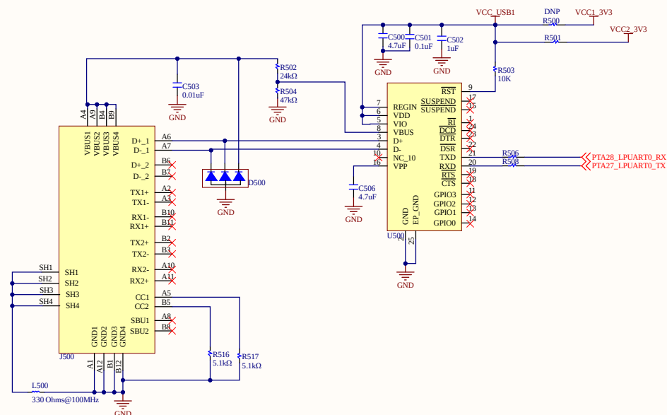
USB TO UART
