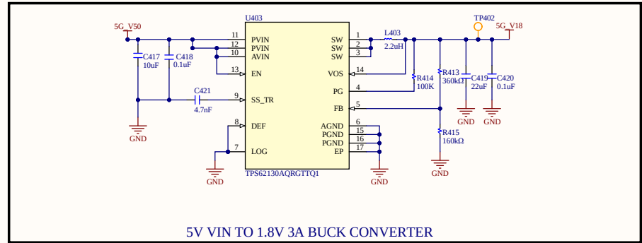
5V VIN TO 1.8V 3A BUCK CONVERTER
