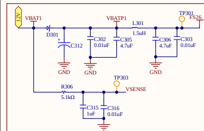
VBAT INPUT FILTER
