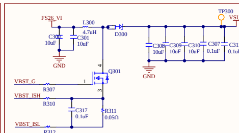
BOOST CIRCUIT
