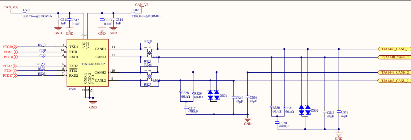
CAN FD TRANSCEIVER
